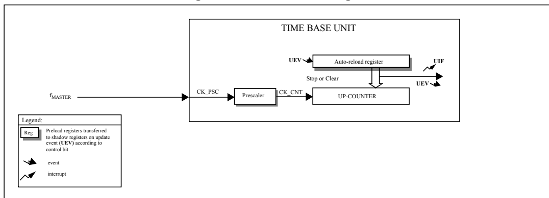
Figure 89. TIM4 block diagram
