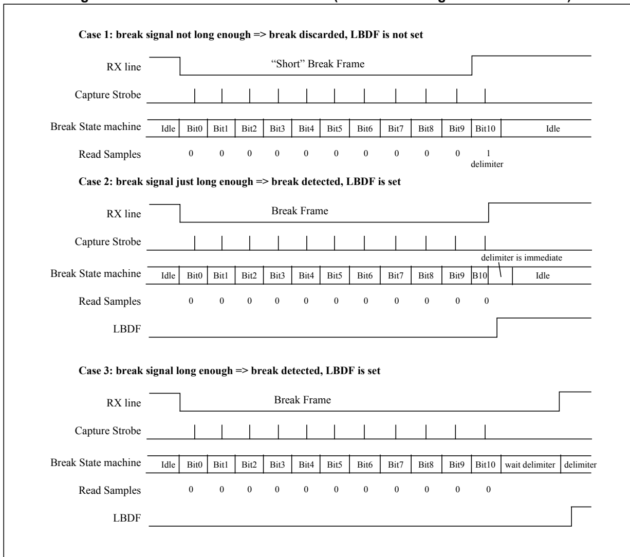
Figure 130. Break detection in LIN mode (11-bit break length - LBDL bit is set)
