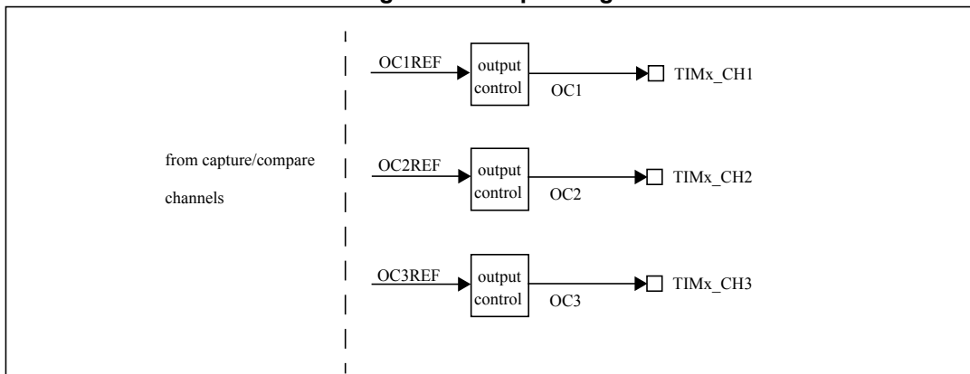
Figure 87. Output stage
