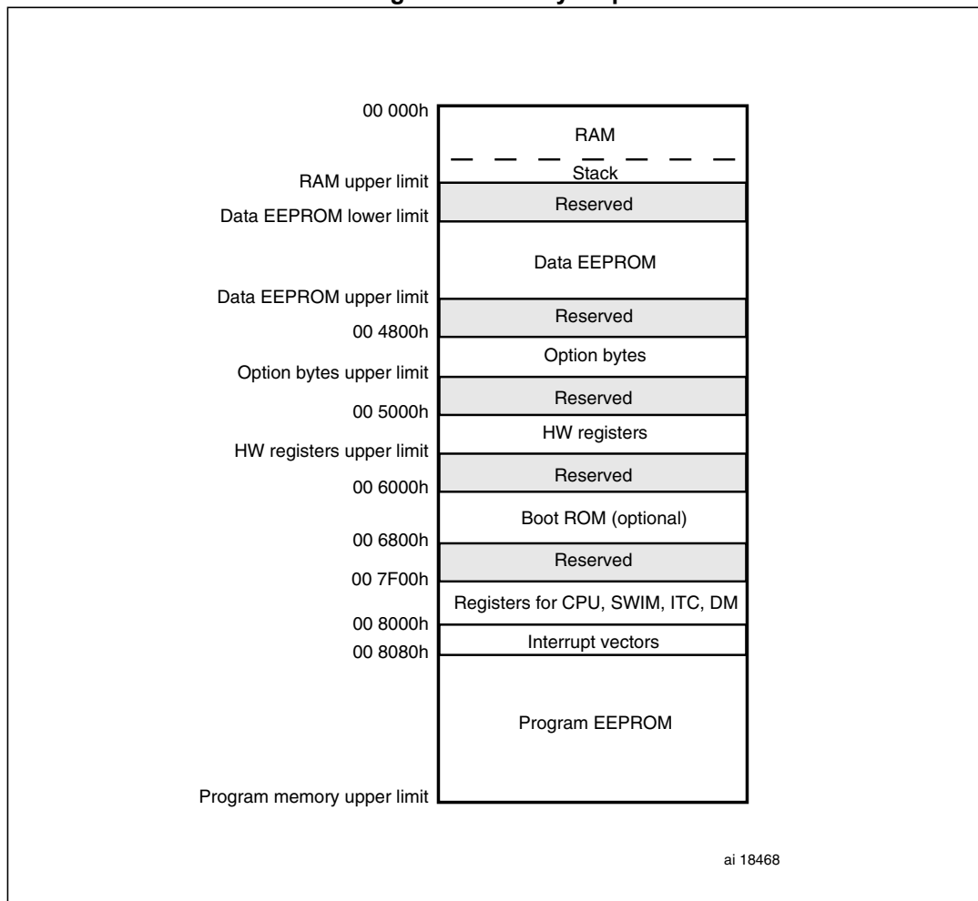
Figure 3. Memory map
