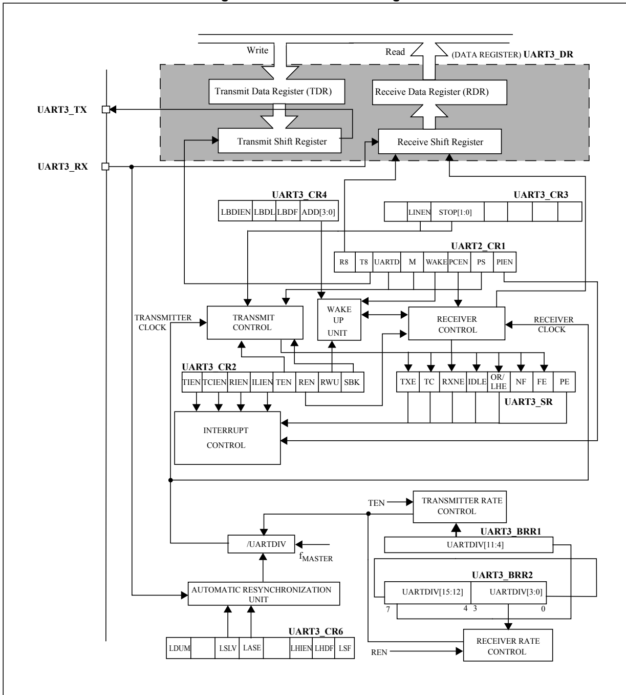
Figure 112. UART3 block diagram
