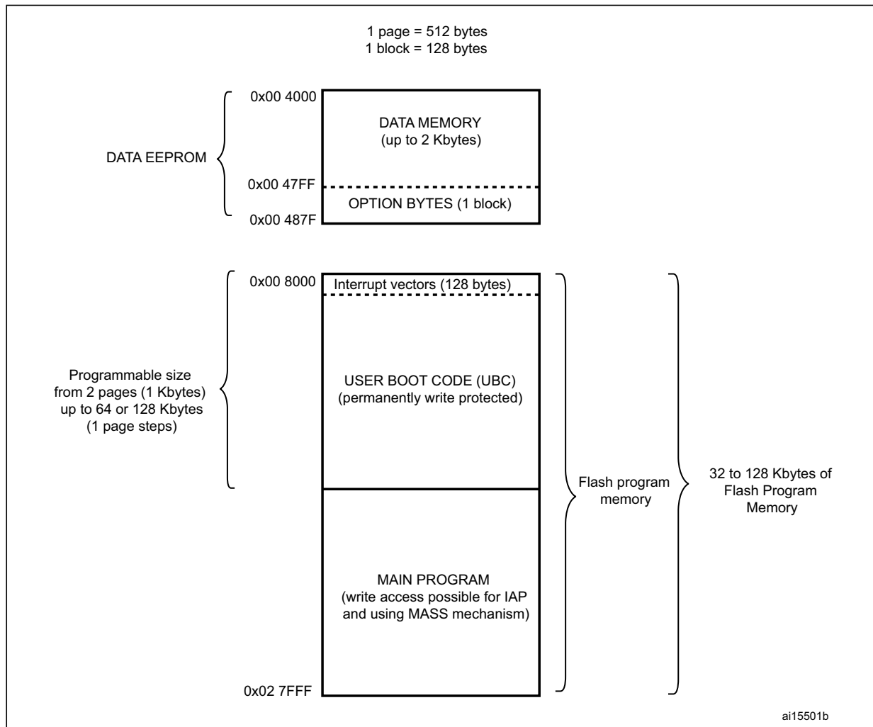
Figure 8. Flash memory and data EEPROM organization high density STM8S and STM8AF
