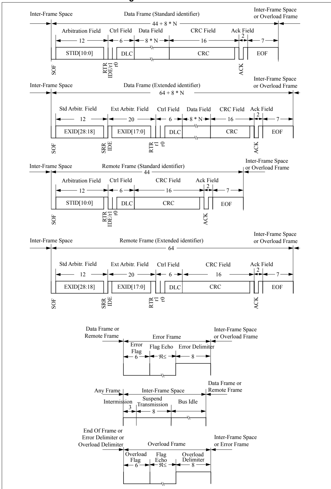
Figure 155. CAN frames
