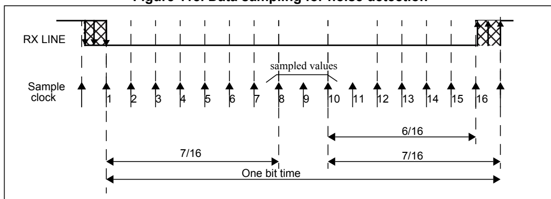
Figure 118. Data sampling for noise detection
