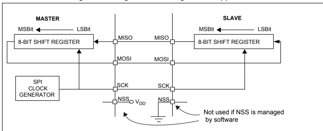
Figure 92. Single master/ single slave application
