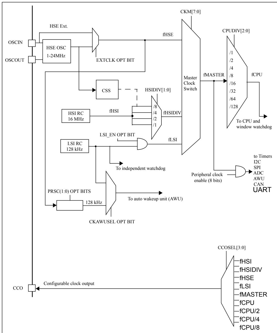
Figure 20. Clock tree
