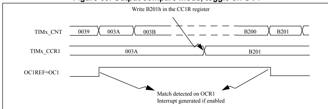
Figure 69. Output compare mode, toggle on OC1
