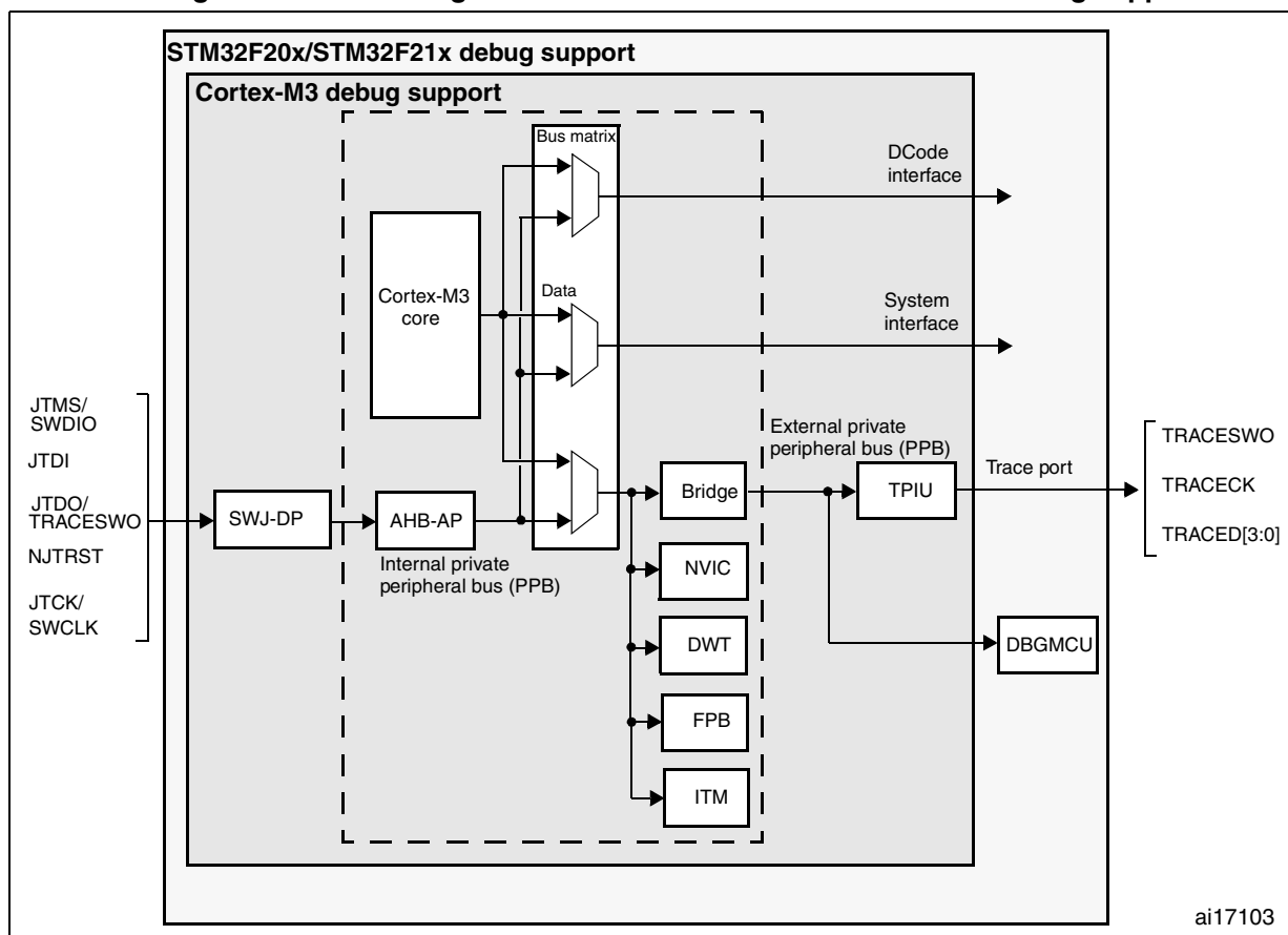
Figure 416. Block diagram of STM32 MCU and Cortex-M3-level debug support
