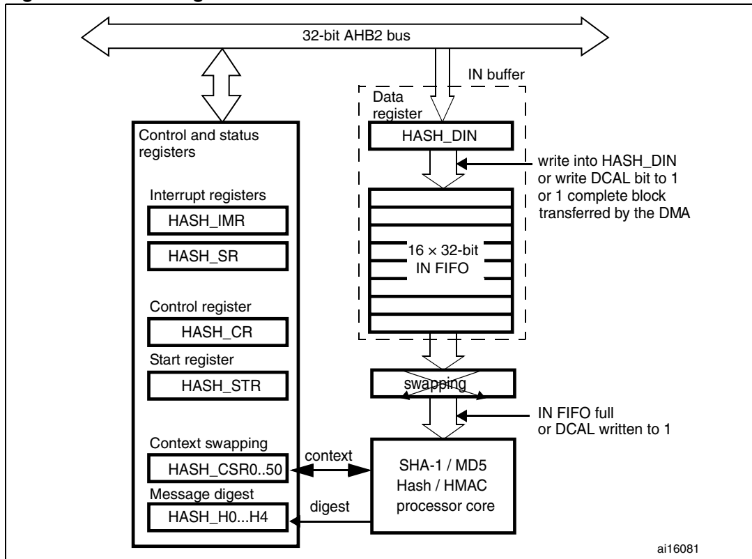
Figure 211. Block diagram
