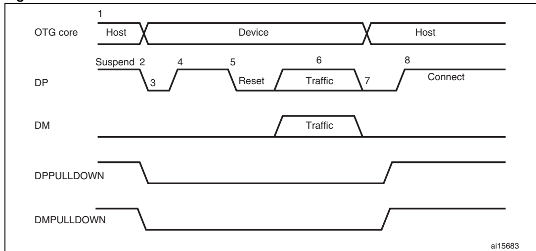
Figure 370. A-device HNP
