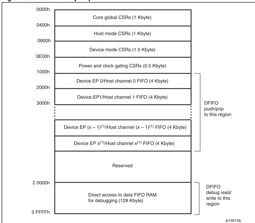
Figure 375. CSR memory map
