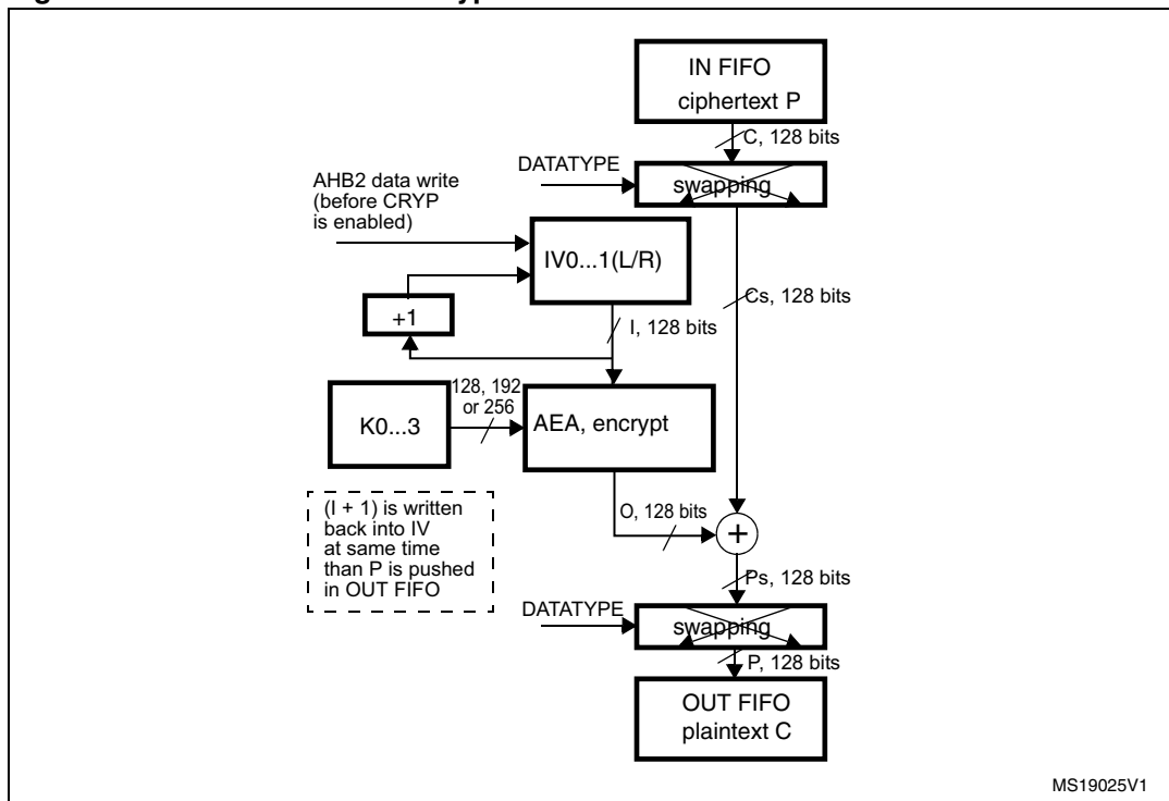
Figure 205. AES-CTR mode encryption
