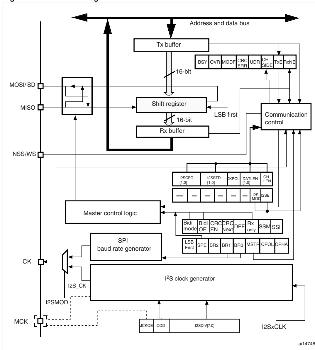
Figure 264. I 2 S block diagram
