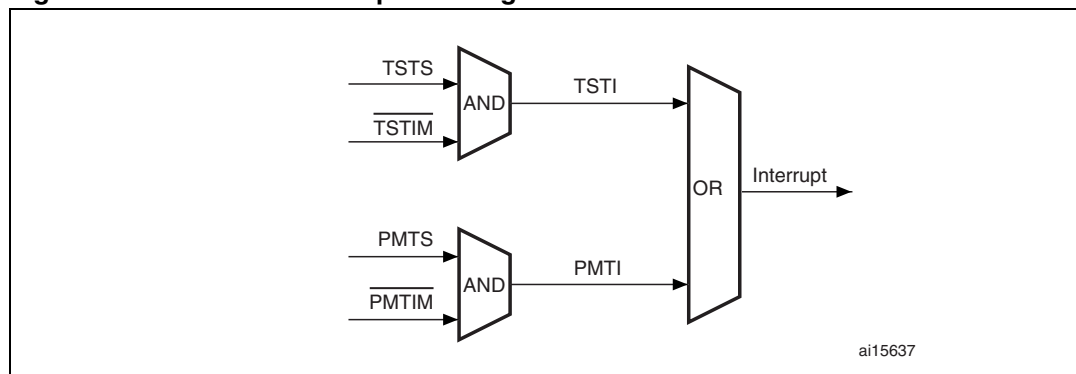
Figure 332. MAC core interrupt masking scheme
