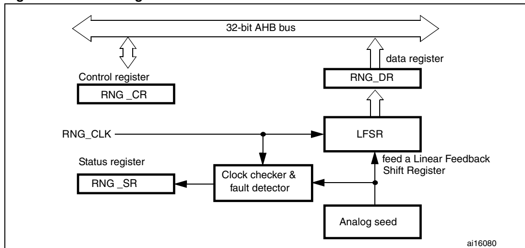
Figure 210. Block diagram
