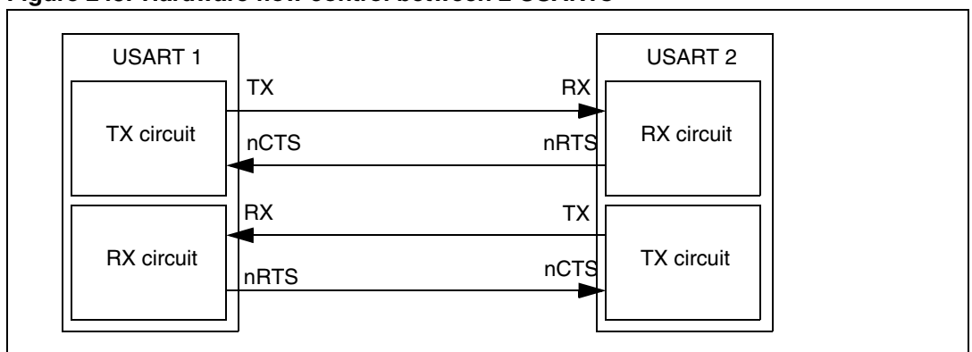
Figure 243. Hardware flow control between 2 USARTs
