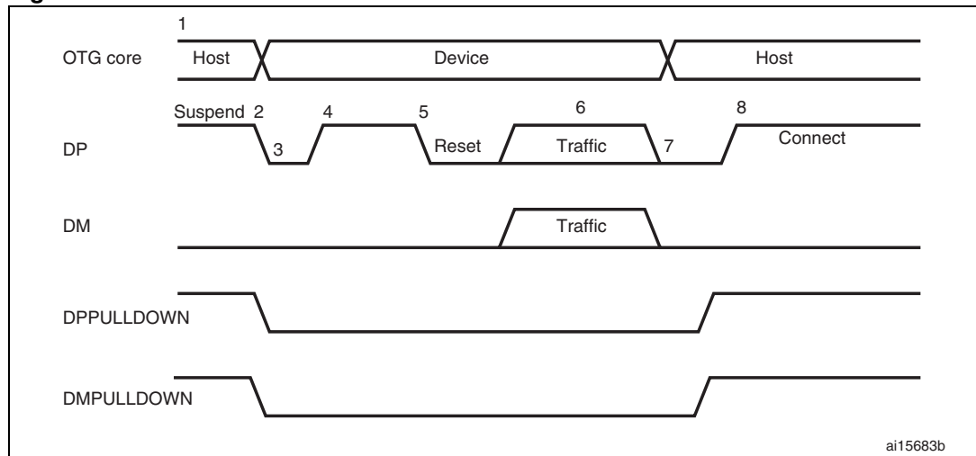
Figure 392. A-device HNP
