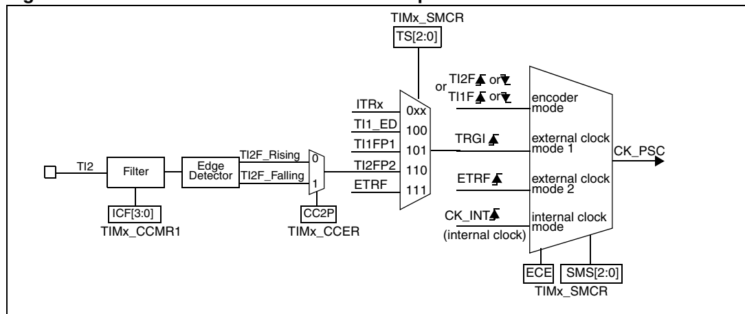
Figure 87. TI2 external clock connection example
