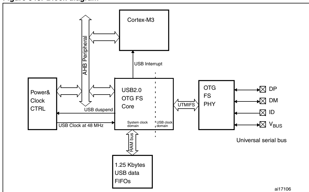
Figure 348. Block diagram
