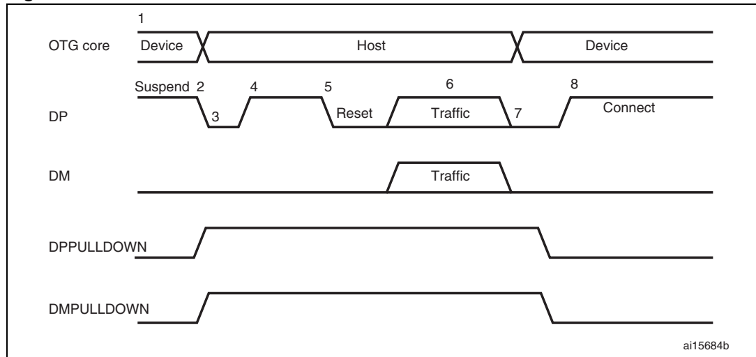
Figure 393. B-device HNP
