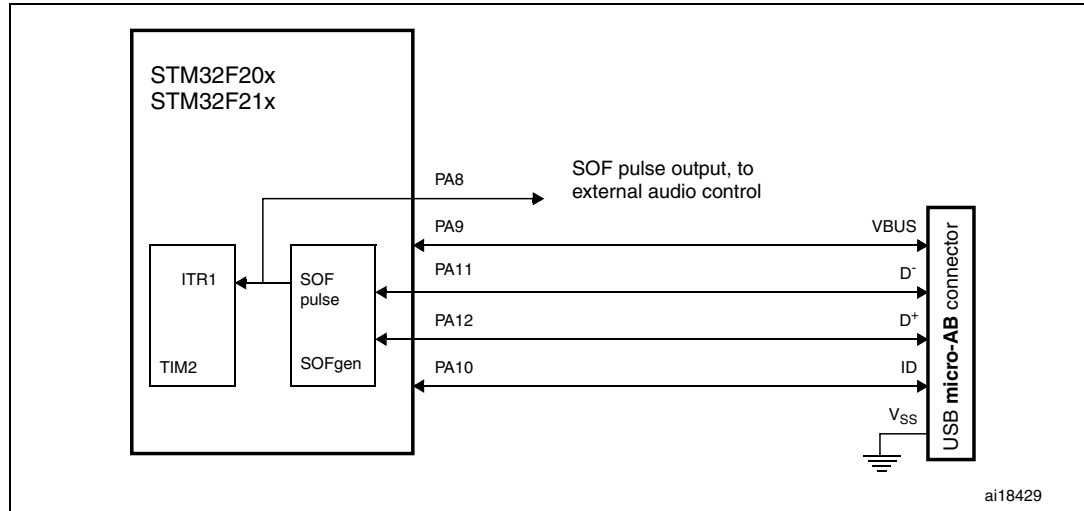
Figure 352. SOF connectivity
