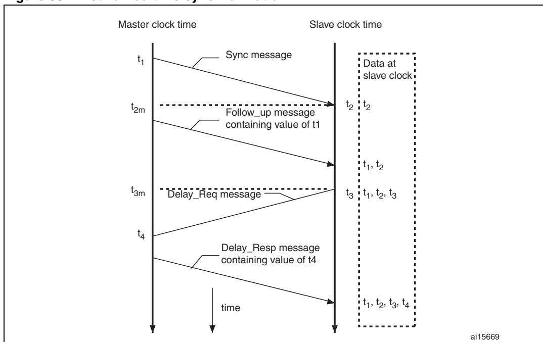
Figure 334. Networked time synchronization
