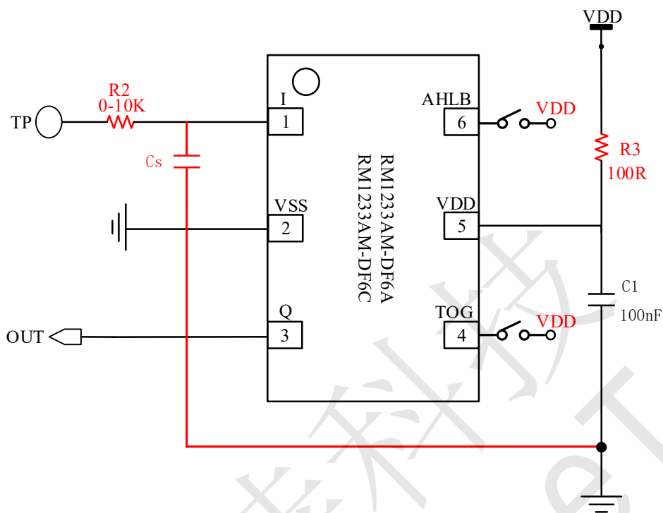
RM1233AM-DF6A/DF6C DFN-6L 应用图
