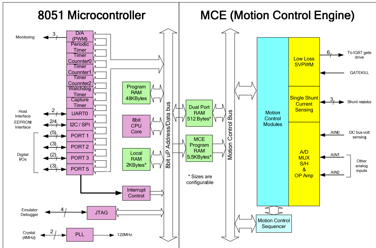
Figure 2. IRMCF371 Internal Block Diagram
