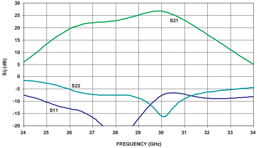
RMDA29000 S-Parameters vs. Frequency 5V, 250mA, T = 25°C
