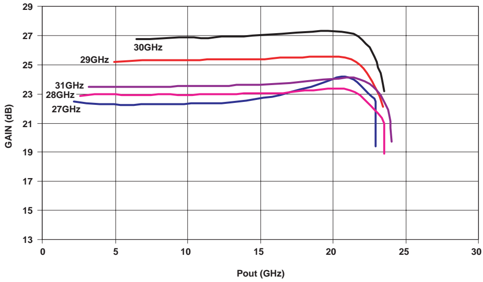
RMDA29000 Gain vs. Pout 5V, 250mA, T = 25°C
