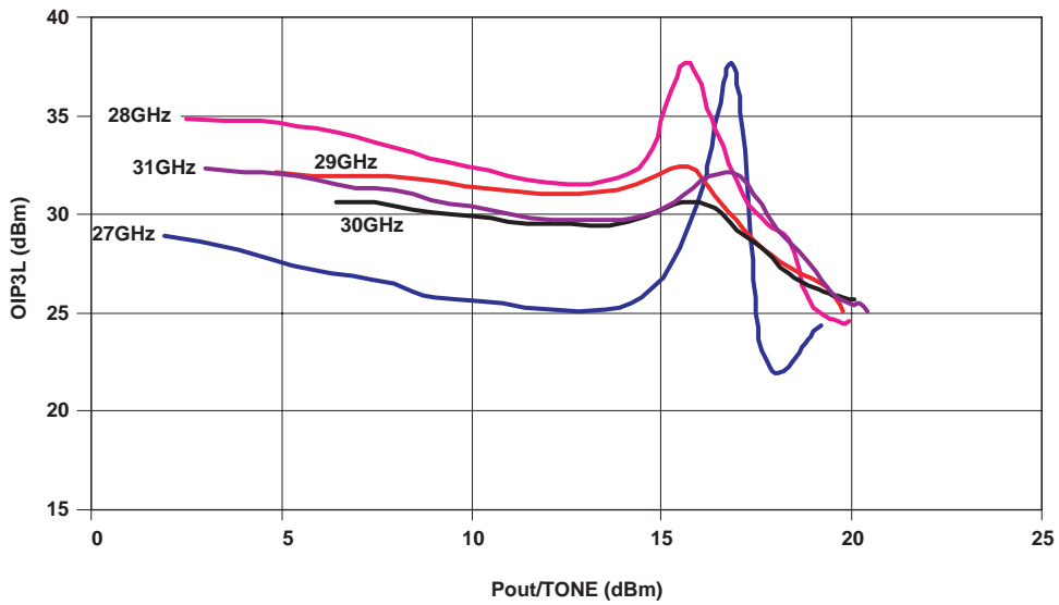
RMDA29000 PIP3 vs. Pout/Tone 10 MHz Tone Sep 5V, 250mA, T = 25°C
