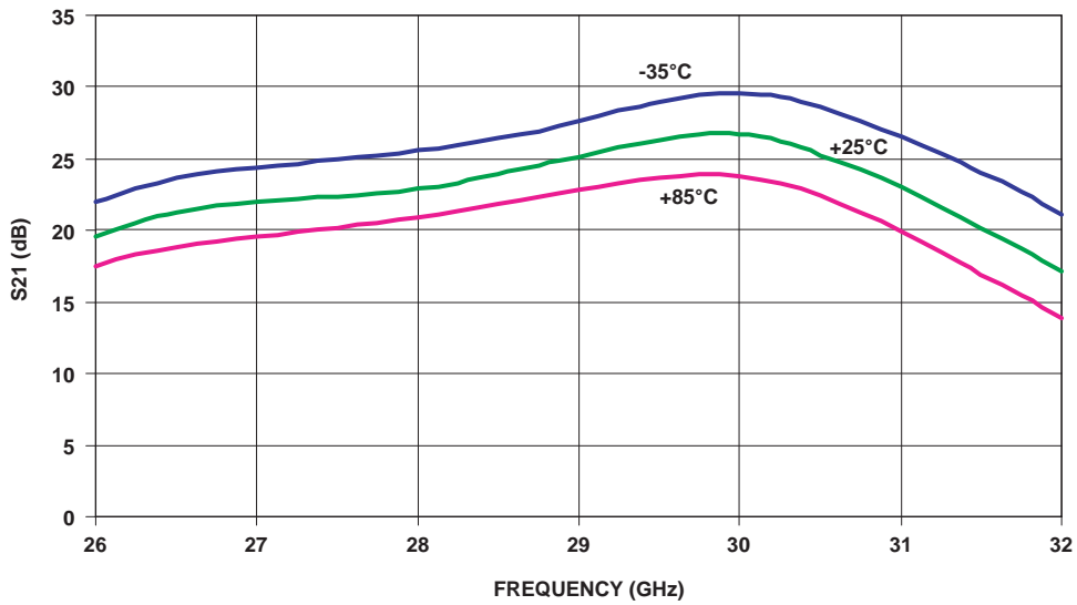
RMDA29000 S21 vs. Frequency Over Temperature 5V, 250mA
