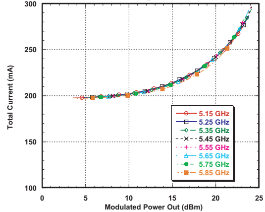
RMPA2550 Total Current Vs. Modulated Pout 5.15 to 5.85 GHz VM, VC=3.3V T=25C Data Rate 54Mbps OFDM 16.7MHz
