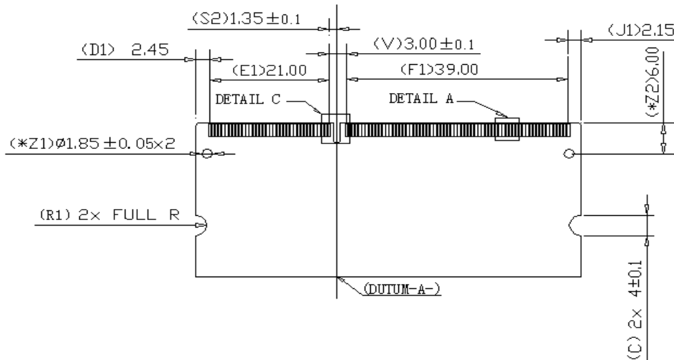
Detail A
