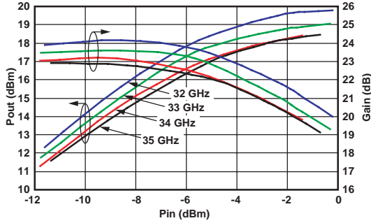
RMWB33001 33 GHz BA, Power Output and Gain vs. Power In 50Ω Fixture Measurements, Vd=4 V, Idq = 112 mA, T=25°C
