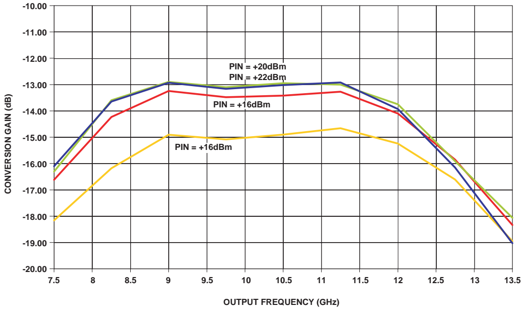
RMWT04001, 4 to 12 GHz Tripler, Typical Performance, Chip Bonded into 50Ω Test Fixture
