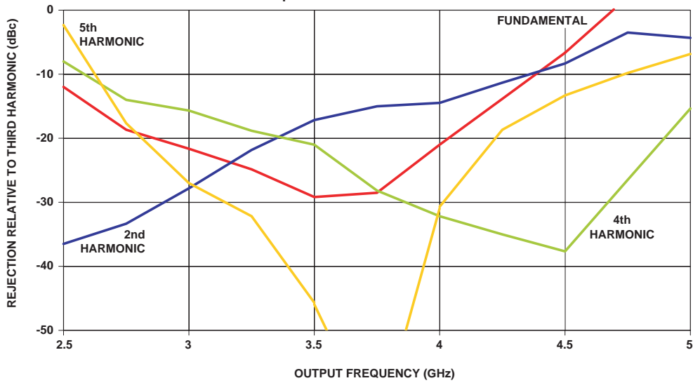
RMWT04001, 4 to 12 GHz Tripler, Typical Performance, Chip Bonded into 50Ω Test Fixture
