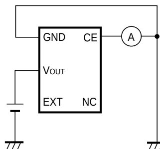
Test Circuit 8
