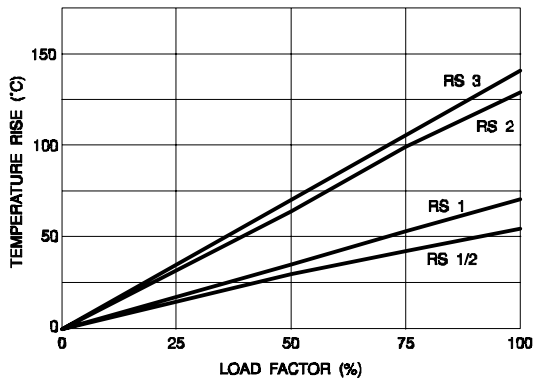
Surface Temperature Rise vs. Load - Type RS
