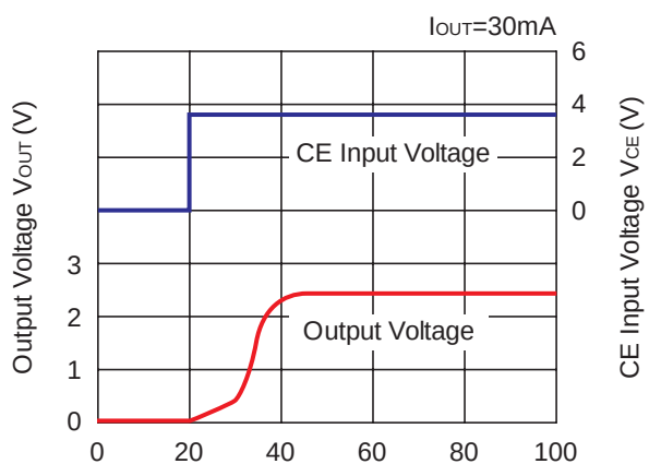
RP100x251x
