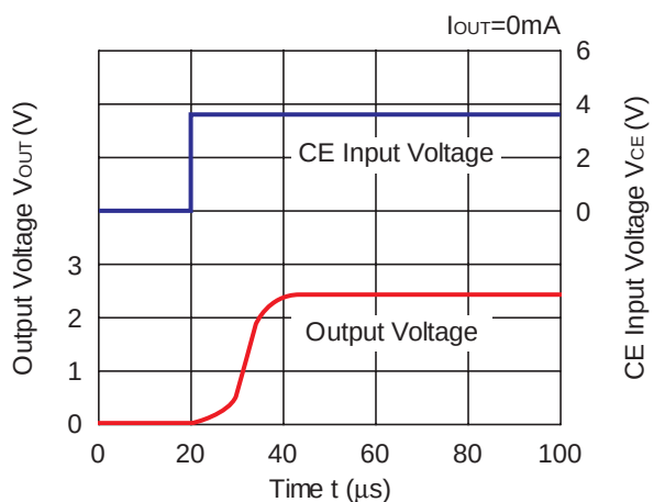
RP100x251x
