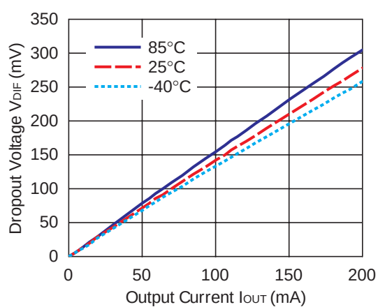
RP100x171x
