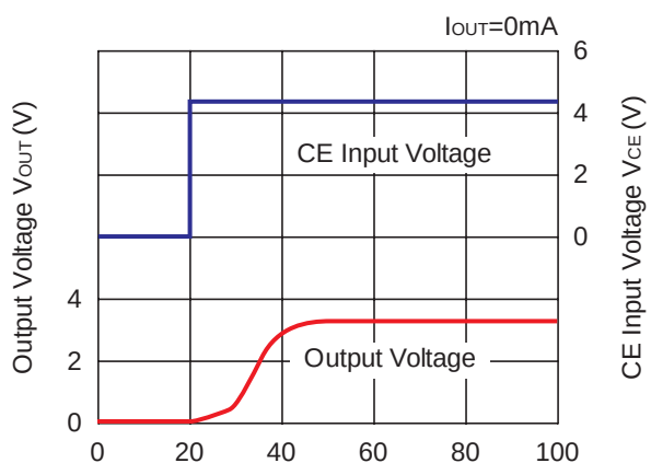
RP100x331x
