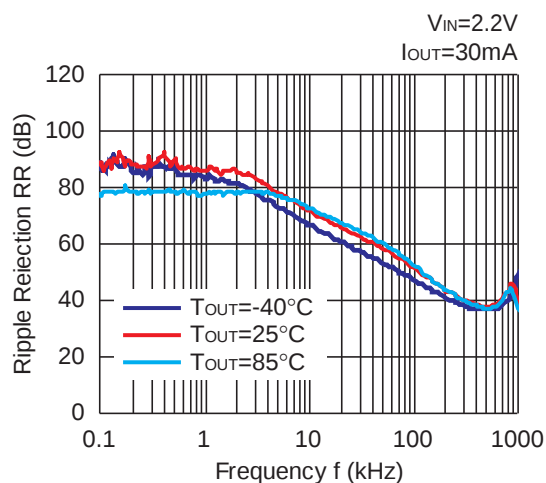
RP102x121x
