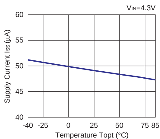
RP102x331x
