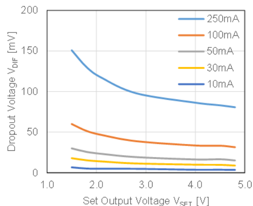
RP123K/Nxx1x
