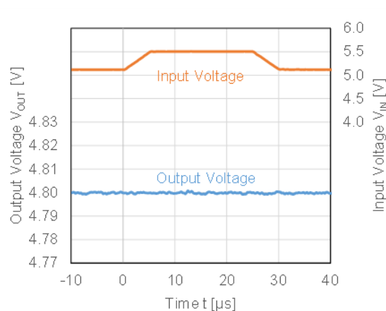
RP123x48xx, I_{OUT} = 20 \text{ mA}
