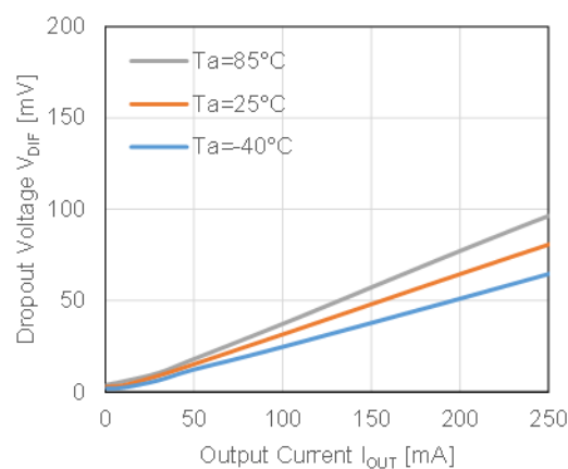
RP123K/N481x
