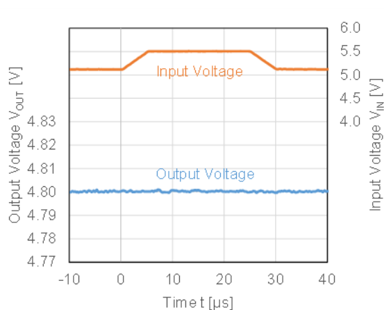
RP123x48xx, I_{OUT} = 1 \text{ mA}
