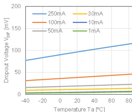
RP123K/N281x
