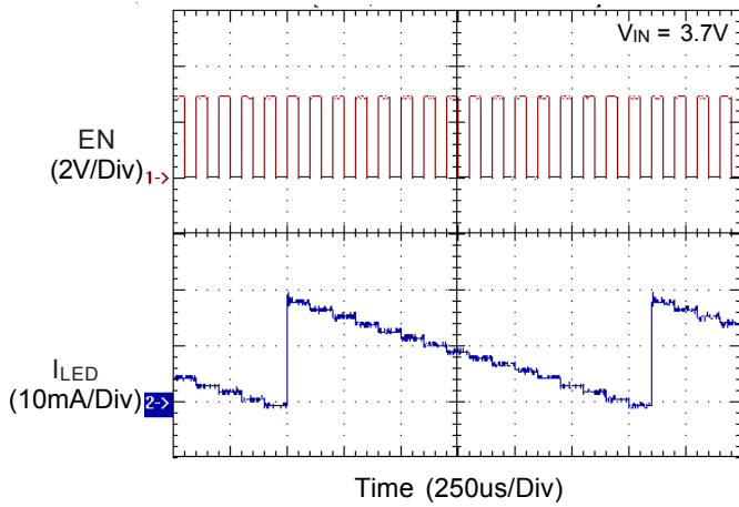
Dimming Operation
