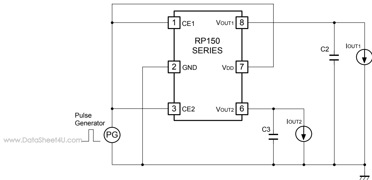
Test Circuit for Ripple Rejection
