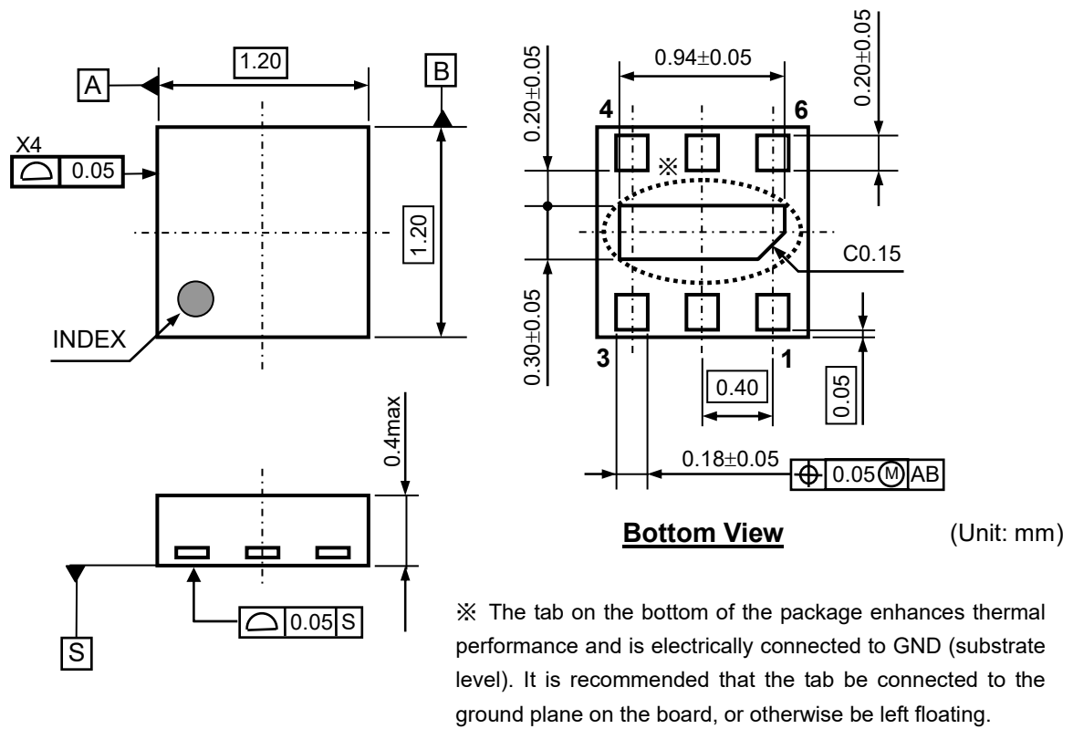
DFN1212-6 Package Dimensions
