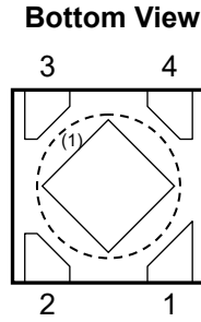
RP173K [DFN(PL)1010-4] Pin Configuration
