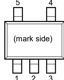
RP173N (SOT-23-5) Pin Configuration
