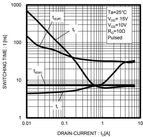
Fig.11 Switching Characteristics
