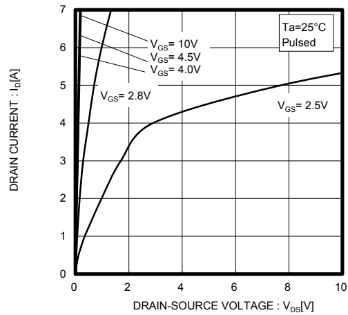
Fig.2 Typical Output Characteristics( II )
