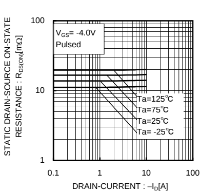
Fig.7 Static Drain-Source On-State Resistance vs. Drain Current
