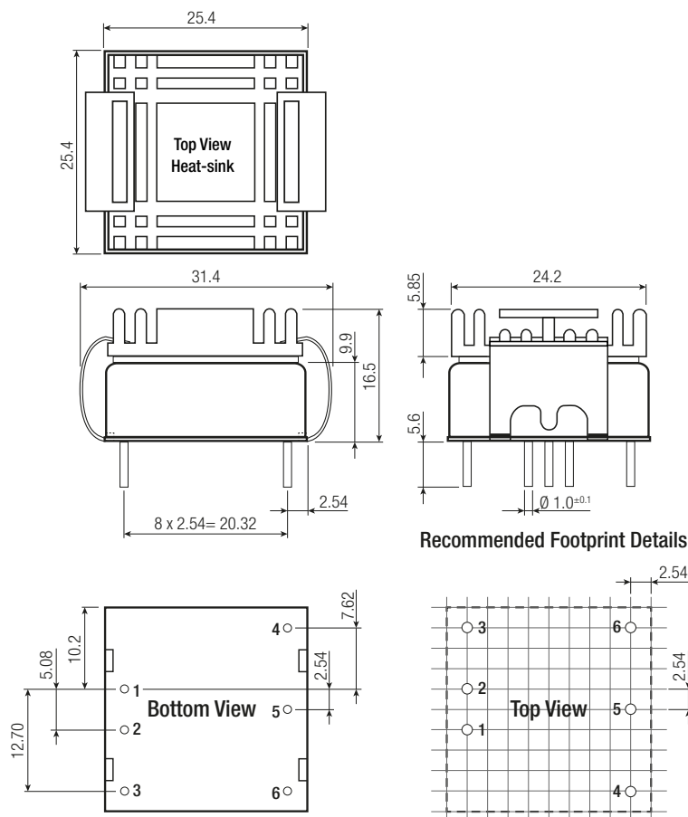
Dimension Drawing (mm) with Heat-sink
