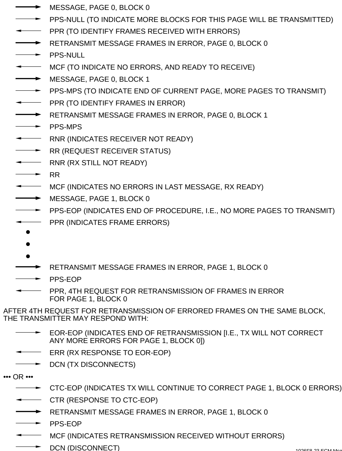
Figure 8-23. ECM Message Protocol Example
