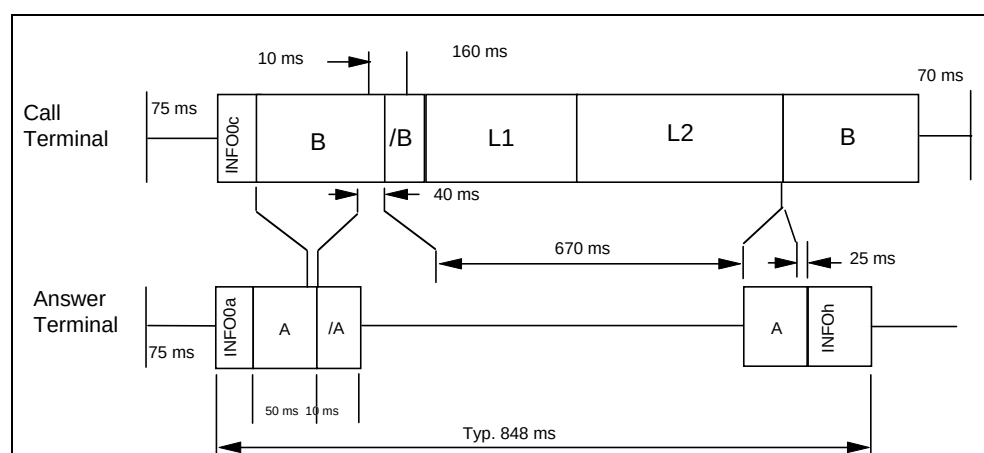
Figure 17-3. V.34 Line Probing (Phase 2)
