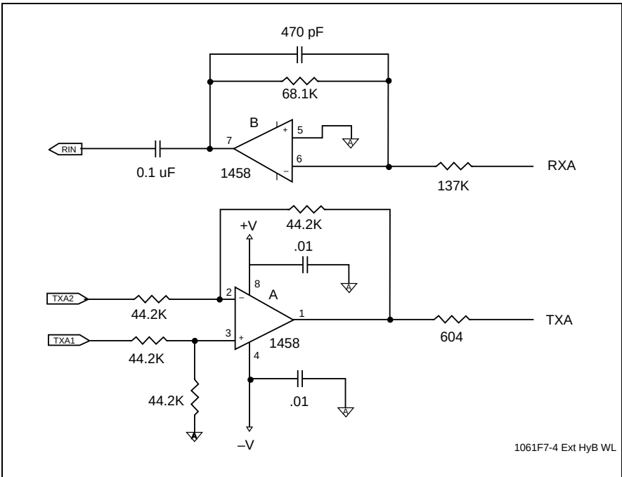
Figure 7-2. Typical Interface to External Hybrid
