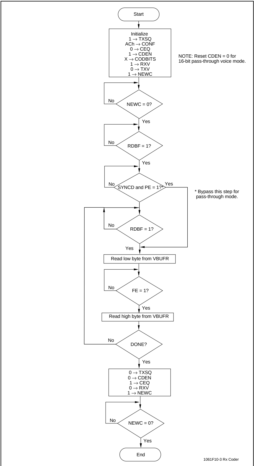
Figure 11-3. Rx-Coder Operation
