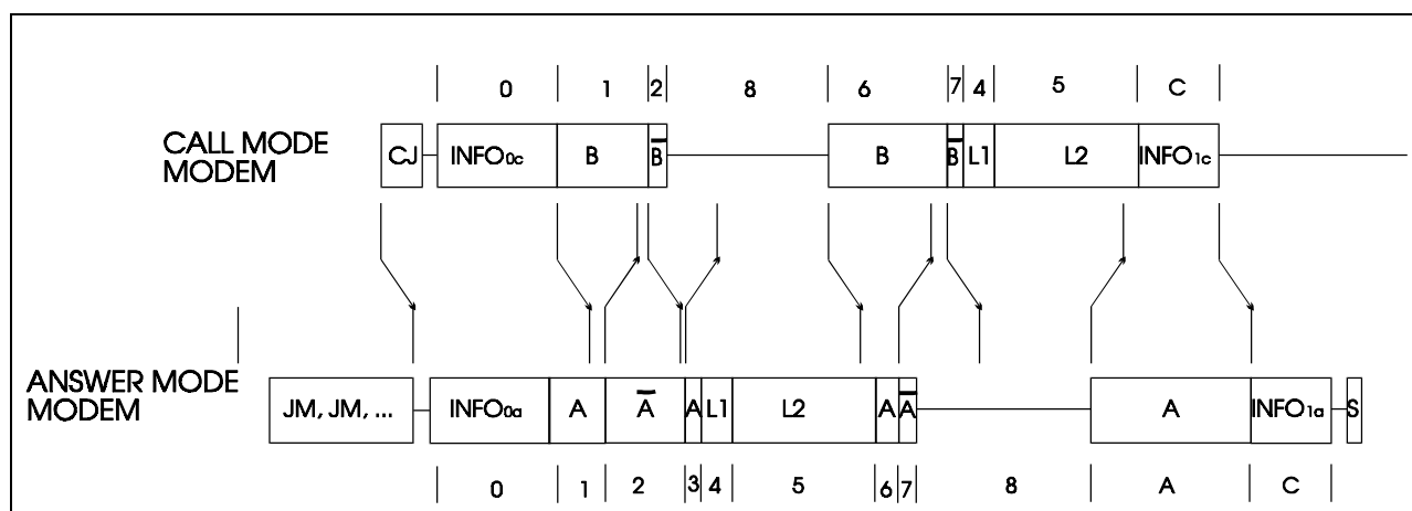
Figure 9-2. Phase 2 Transmitter States
