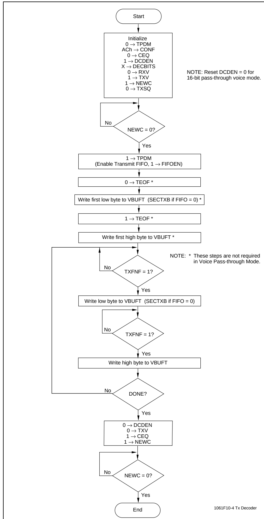
Figure 11-4. Tx-Decoder Operation
