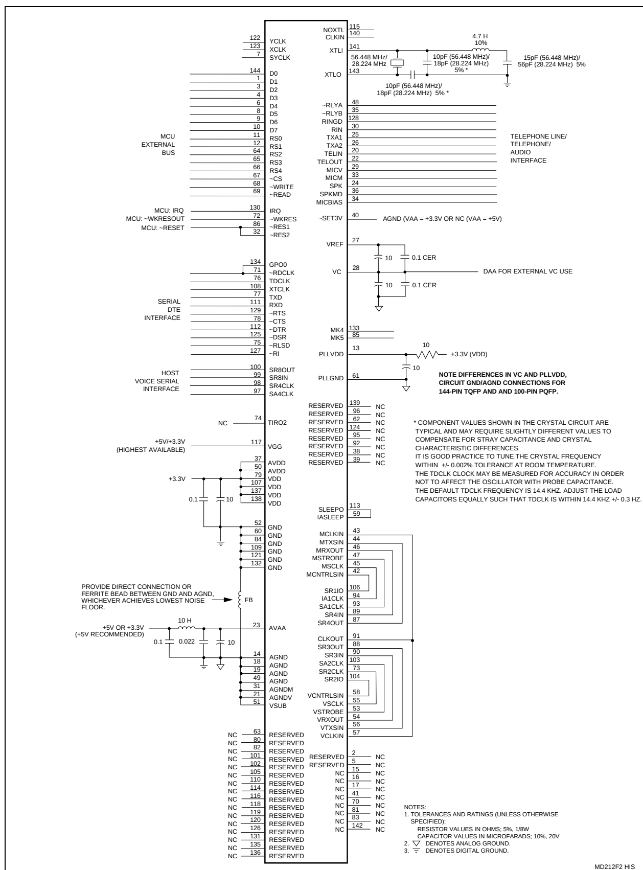
Figure 2-2. MDP Hardware Interface Signals-144-Pin TQFP
