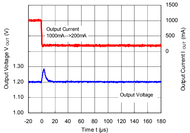
RP506Kxx1A/B/C ( V_{IN} = 3.6\text{ V} , V_{OUT} = 1.2\text{ V} )
