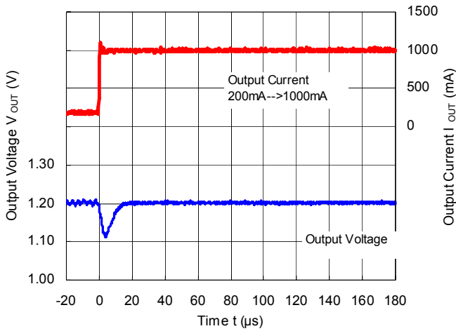
RP506Kxx1A/B/C ( V_{IN} = 3.6\text{ V} , V_{OUT} = 1.2\text{ V} ) MODE = "H" Forced PWM Control
