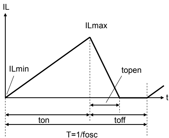
Figure 1. Discontinuous Mode
