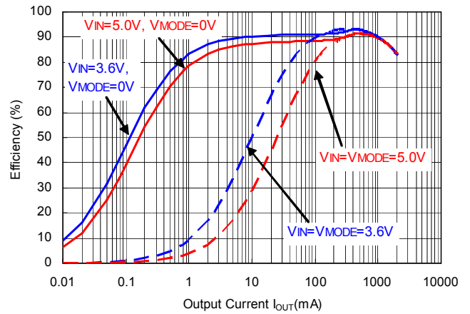
RP506Kxx1D/E/F V_{OUT} = 1.8 V
