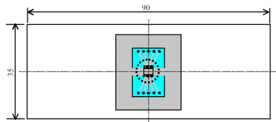
High Wattage Land Pattern
