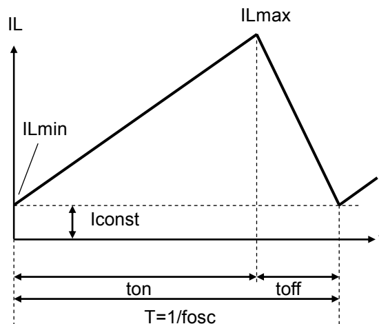
Figure 2. Continuous Mode
