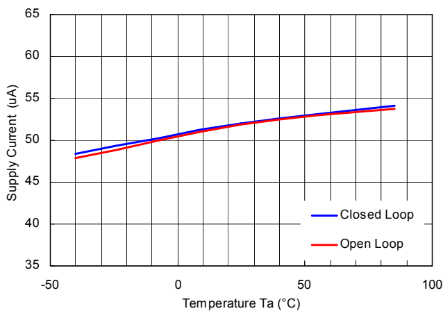
RP506 K V_{OUT} = 1.8 V (V_{IN} = 5.5 V) MODE = "L" PWM/VFM Auto Switching Control
