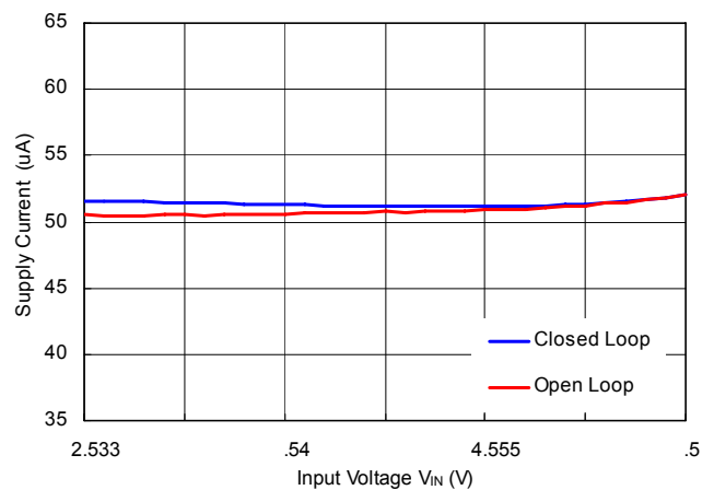
RP506K V_{OUT} = 1.8 V MODE = "L" PWM/VFM Auto Switching Control
