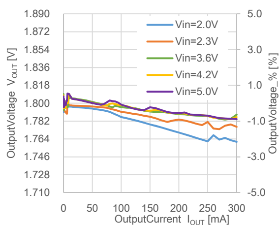
RP512x181x, T_a = 25^\circ\text{C}
