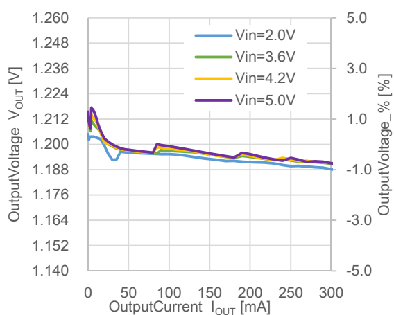
RP512x331x, T_a = 25^\circ\text{C}
