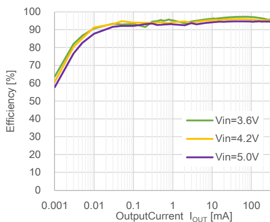
RP512x121x, T_a = 25^\circ\text{C}
