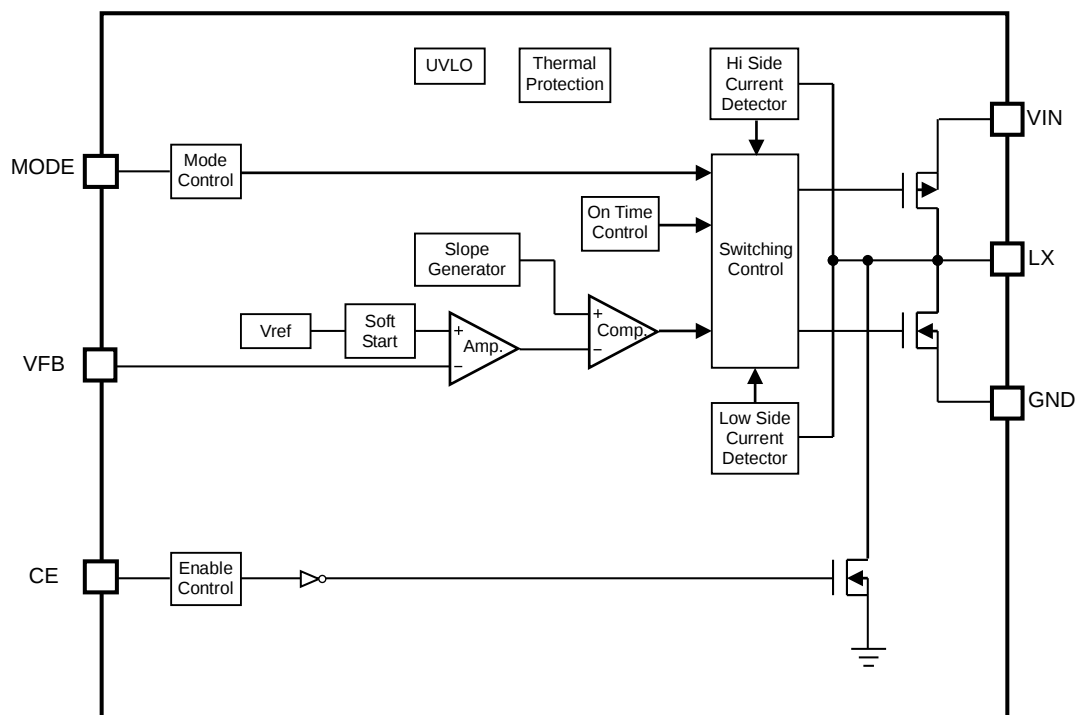
RP519Z00XD Block Diagram
