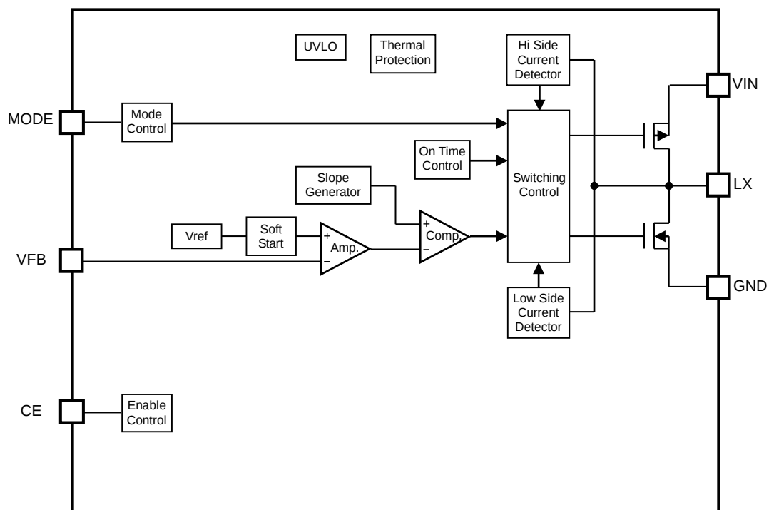
RP519Z00XC Block Diagram
