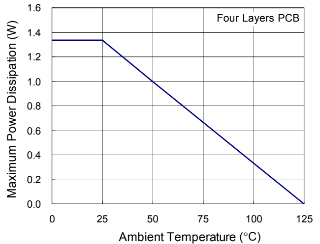
Figure 3. Derating Curve for RP6001 Package
