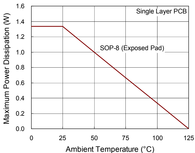
Figure 7. Derating Curves for RP6104 Package
