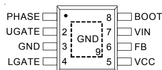
SOP-8 (Exposed Pad)
