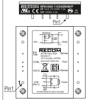
Pin1 identification
