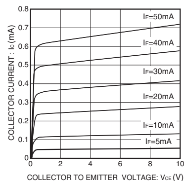
Fig.9 Output characteristics
