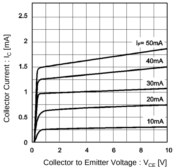
Fig.10 Output Characteristics
