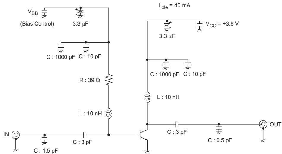
Evaluation Board Circuit
