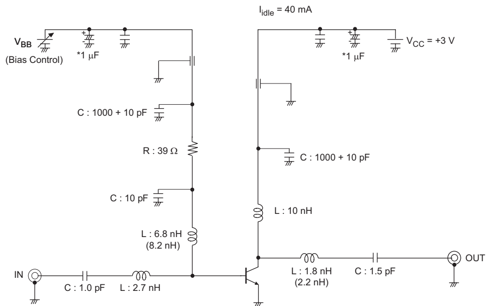
Evaluation Board Circuit
