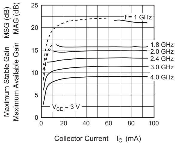
Maximum Available Gain, Maximum Stable Gain vs. Collector Current
