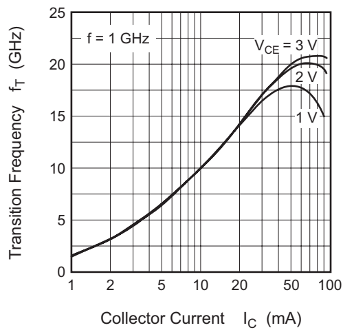
Transition Frequency vs. Collector Current
