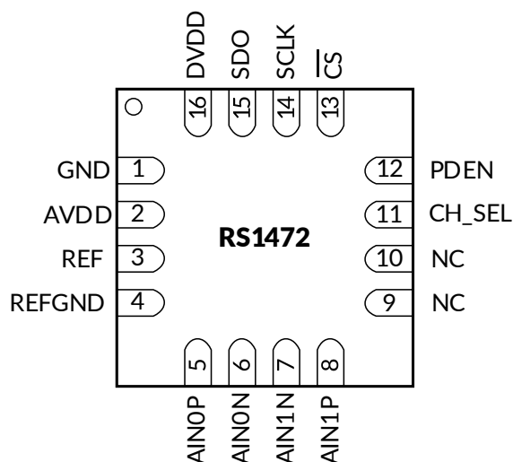
Figure 2. QFN3x3-16
