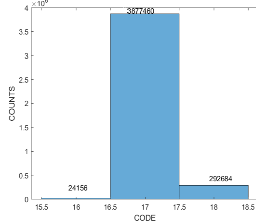
Figure 42. Histogram of a DC Input near Code Center
