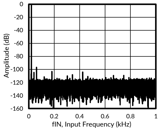
Figure 45. 20 kHz FFT, VREF = 2.5\text{ V}
