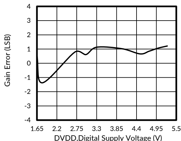
Figure 16. GAIN ERROR vs DIGITAL SUPPLY VOLTAGE
