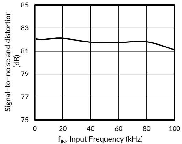
Figure 28. SINAD vs INPUT FREQUENCY
