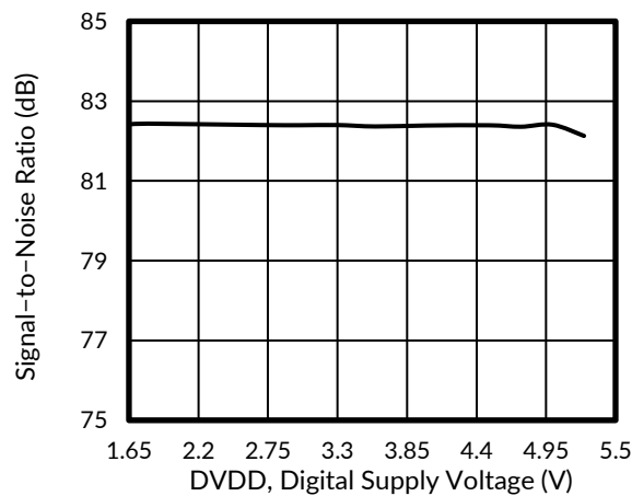
Figure 20. SNR vs DIGITAL SUPPLY VOLTAGE
