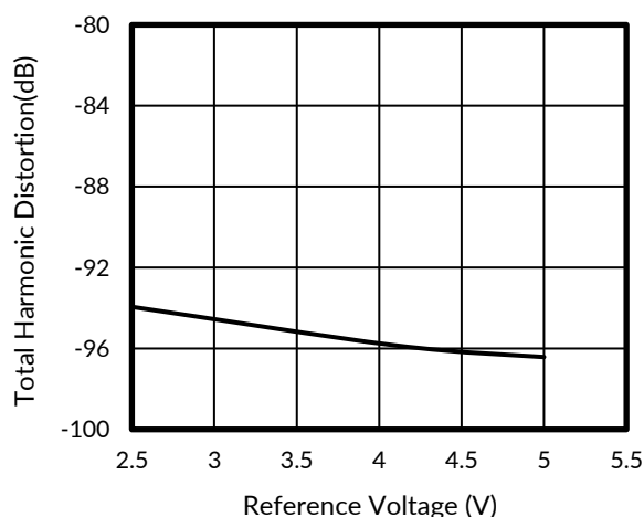
Figure 36. THD vs REFERENCE VOLTAGE
