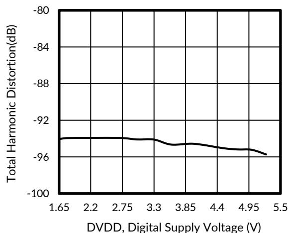
Figure 35. THD vs DIGITAL SUPPLY VOLTAGE
