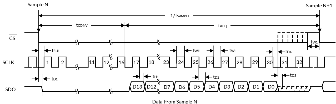
Figure 52. RS1473 Operation in 32-Clock Frame without Power-Down (PDEN = 0)
