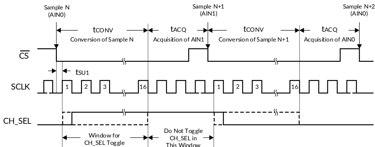
Figure 48. ADC Analog Input Channel Selection
