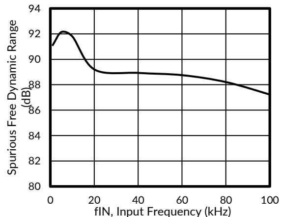
Figure 38. SFDR vs INPUT FREQUENCY
