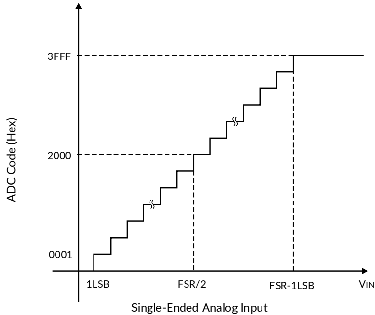
Figure 50. RS1473 Transfer Characteristics
