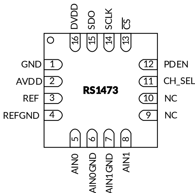
Figure 2. QFN3x3-16
