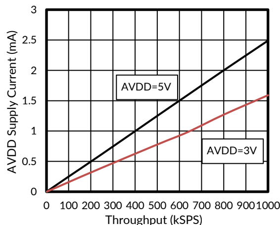
Figure 40. ANALOG SUPPLY CURRENT (Dynamic) vs SAMPLE RATE
