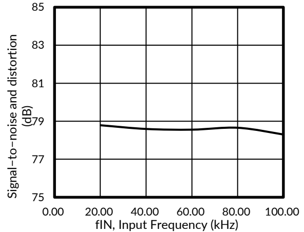
Figure 28. SINAD vs INPUT FREQUENCY
