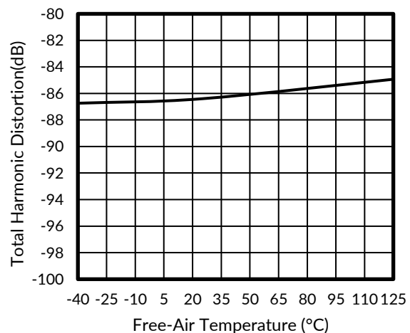
Figure 32. THD vs Free-Air Temperature
