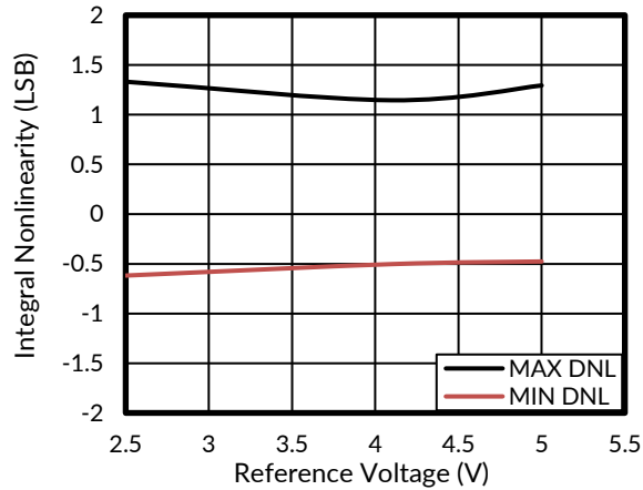
Figure 9. INL vs REFERENCE VOLTAGE
