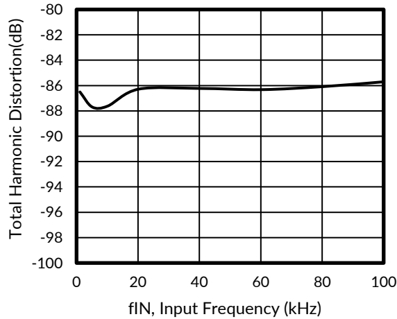
Figure 33. THD vs INPUT FREQUENCY
