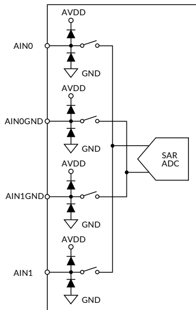
Figure 46. Analog Inputs
