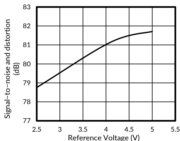
Figure 26. SINAD vs REFERENCE VOLTAGE
