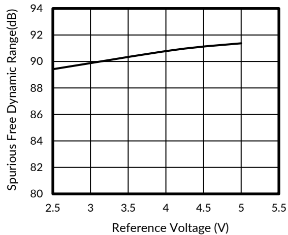
Figure 36. SFDR vs REFERENCE VOLTAGE
