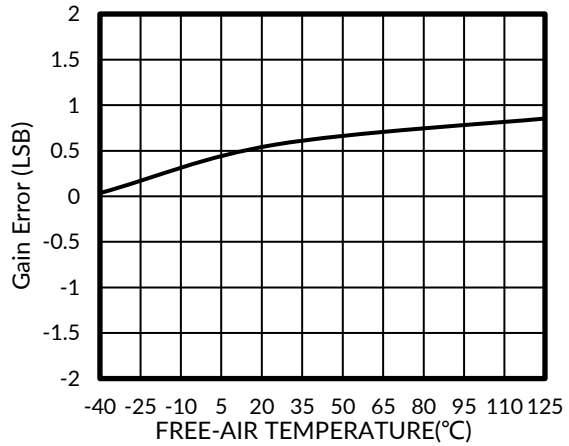
Figure 18. GAIN ERROR vs FREE-AIR TEMPERATURE
