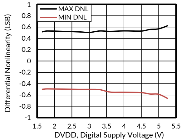
Figure 4. DNL vs DIGITAL SUPPLY VOLTAGE
