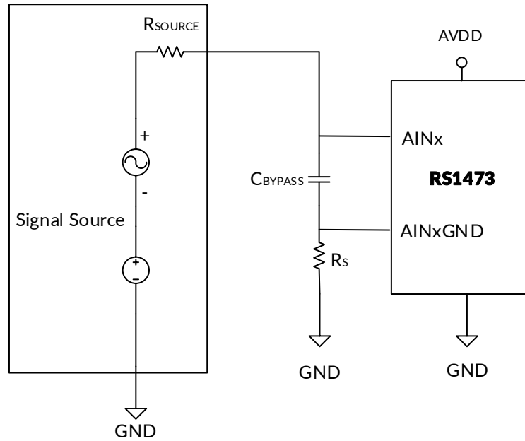
Figure 57. Driving an RS1473 ADC Without a Driving Op Amp
