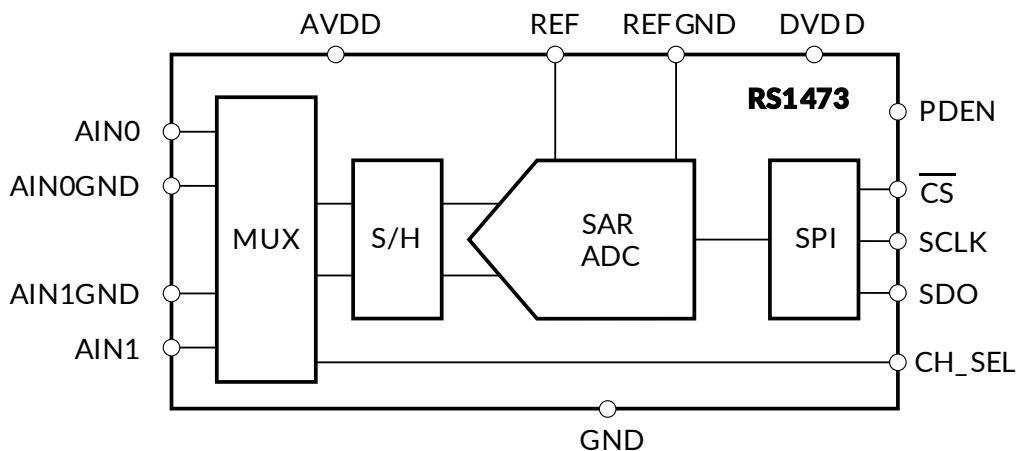
Figure 1. Block Diagram
