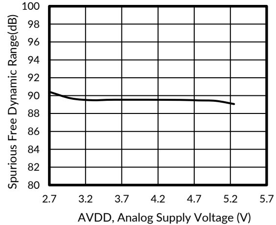
Figure 34. SFDR vs ANALOG SUPPLY VOLTAGE
