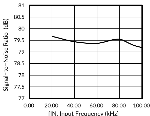
Figure 23. SNR vs INPUT FREQUENCY
