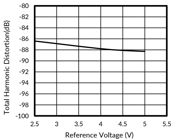
Figure 31. THD vs REFERENCE VOLTAGE
