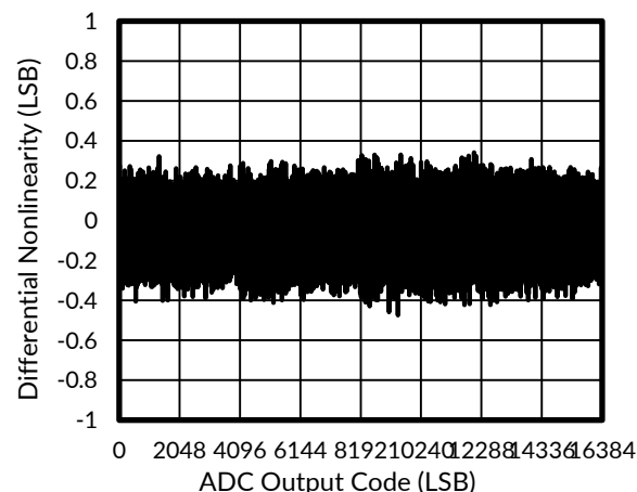
Figure 43. Differential Nonlinearity vs Code
