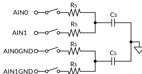
Figure 47. Input Sampling Stage Equivalent Circuit
