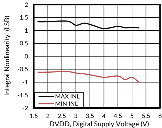
Figure 8. INL vs DIGITAL SUPPLY VOLTAGE
