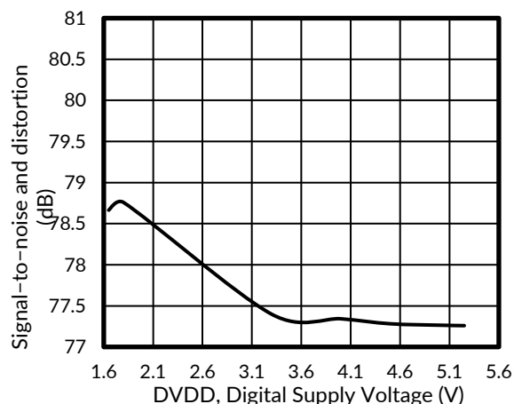
Figure 25. SINAD vs DIGITAL SUPPLY VOLTAGE
