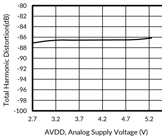
Figure 29. THD vs ANALOG SUPPLY VOLTAGE
