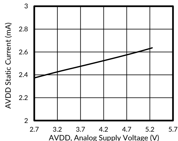
Figure 41. ANALOG SUPPLY CURRENT (Static) vs ANALOG SUPPLY VOLTAGE
