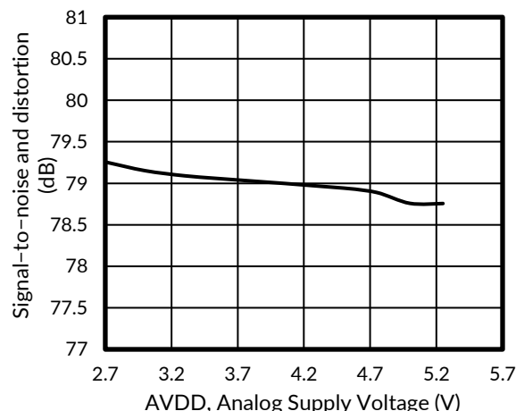
Figure 24. SINAD vs ANALOG SUPPLY VOLTAGE
