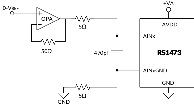
Figure 56. Typical Input Driving Circuit
