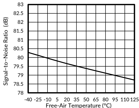
Figure 22. SNR vs Free-Air Temperature
