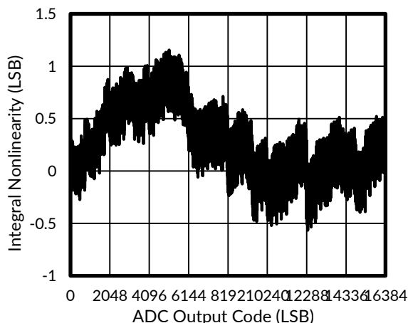
Figure 44. Integral Nonlinearity vs Code
