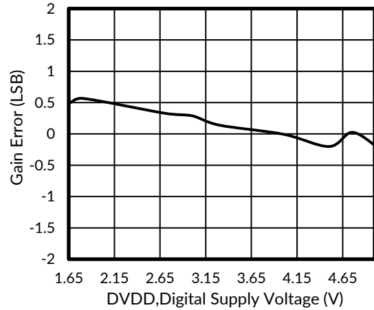
Figure 16. GAIN ERROR vs DIGITAL SUPPLY VOLTAGE
