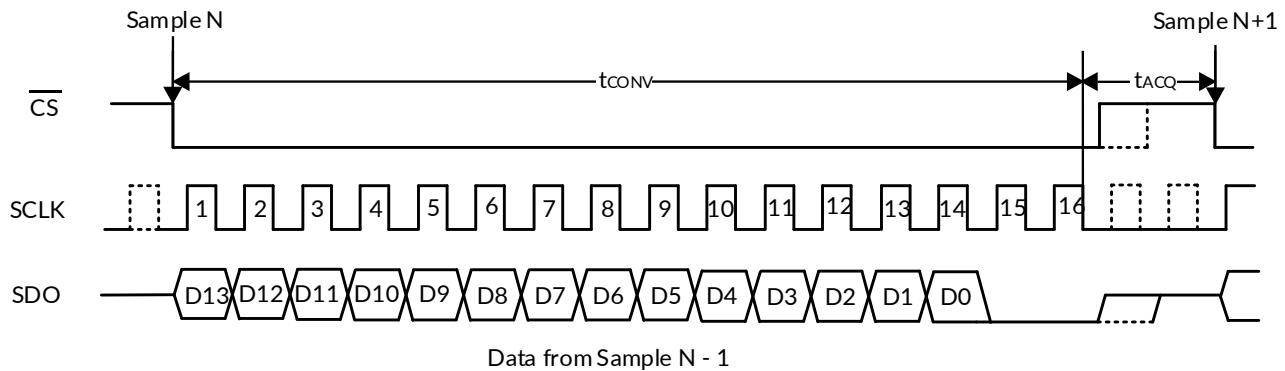
Figure 51. RS1473 Operating in 16-Clock Mode without Power-Down (PDEN = 0)
