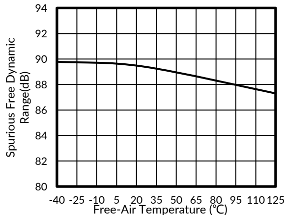
Figure 37. SFDR vs FREE-AIR TEMPERATURE
