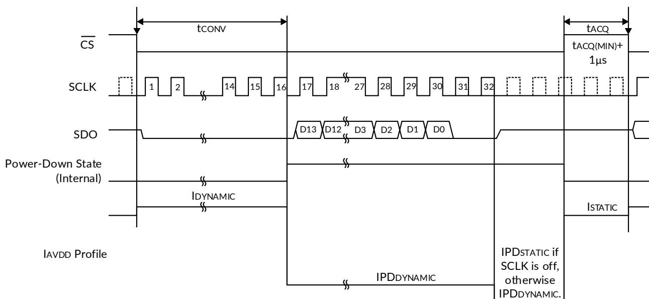
Figure 53. Power-Down Mode (PDEN = 1)
