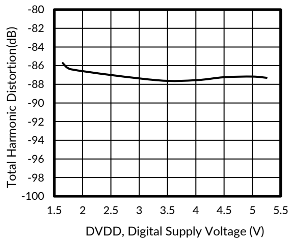
Figure 30. THD vs DIGITAL SUPPLY VOLTAGE
