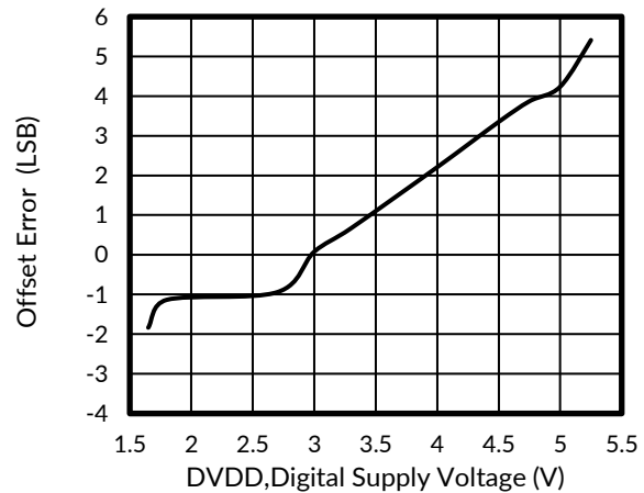
Figure 12. OFFSET ERROR vs DIGITAL SUPPLY VOLTAGE
