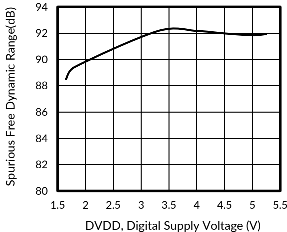
Figure 35. SFDR vs DIGITAL SUPPLY VOLTAGE
