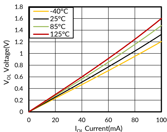
Figure 2. V_{OL} Voltage vs I_{OL} Current
