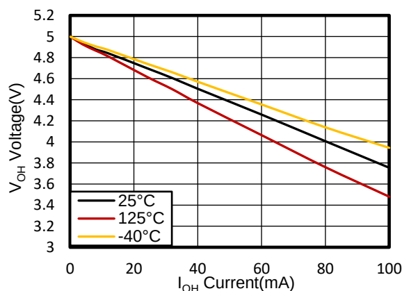
Figure 2. Voltage vs Current
