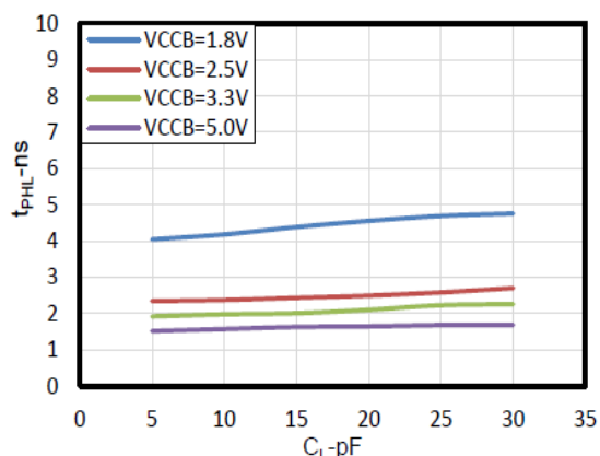
Figure 5. Typical Propagation Delay High-to-Low (A to B) vs Load Capacitance
