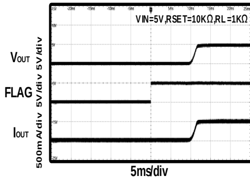
Figure 8. Exit Over Temperature Protection
