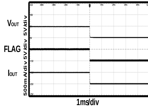
Figure 9. Enter Over Temperature Protection
