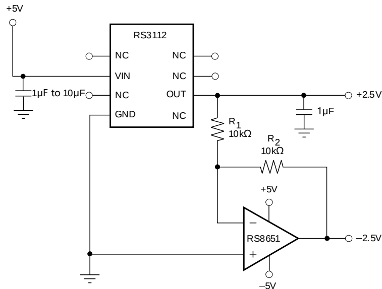
Figure 17. The RS3112 and RS8651 Create Positive and Negative Reference Voltages
