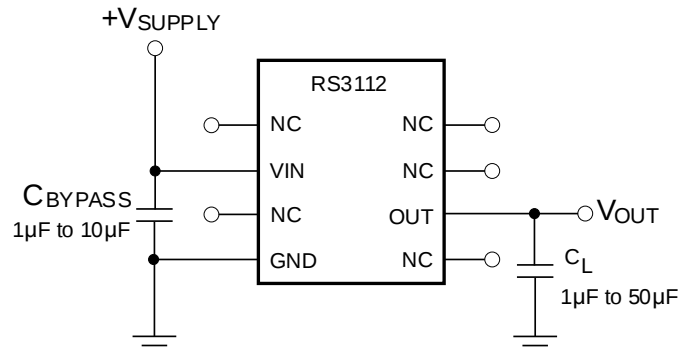
Figure 16. Basic Connections
