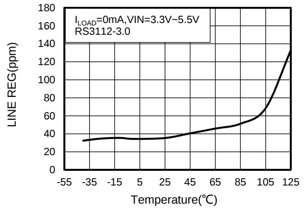
Figure 14. LINE Regulation vs Temperature
