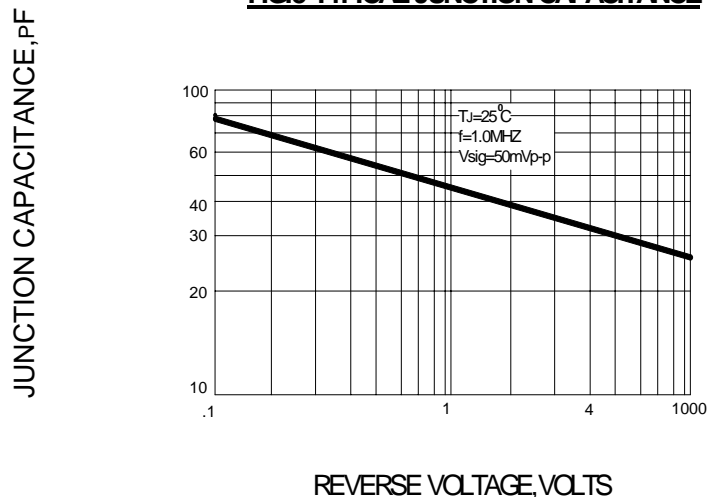
FIG.5-TYPICAL JUNCTION CAPACITANCE
