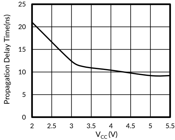
Figure 1. TPD vs V_{CC}
