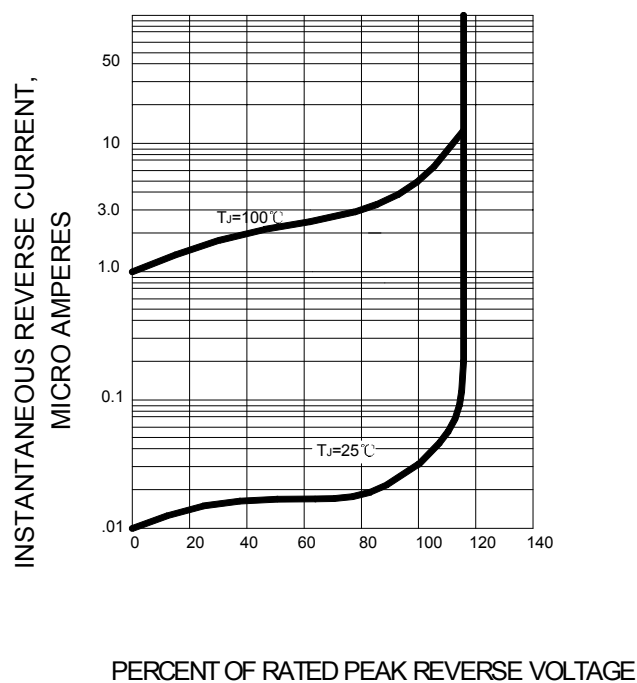
FIG.4 – TYPICAL REVERSE CHARACTERISTIC
