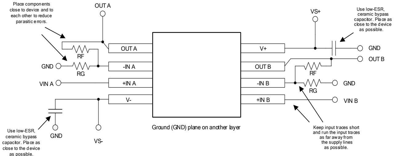
Figure 20. Layout Example
