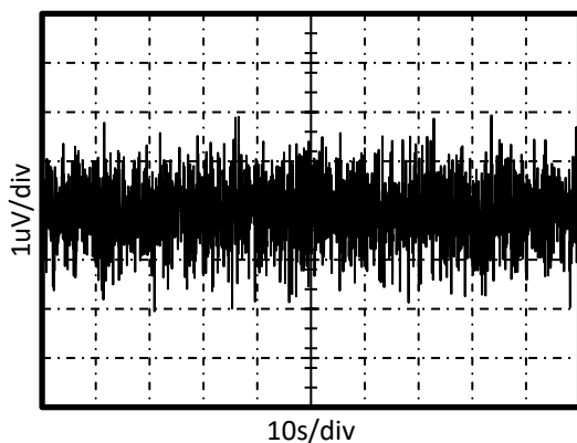
0.01Hz TO 10Hz NOISE AT V_S = 5\text{V}
