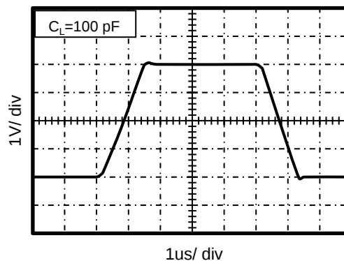
Figure 8. Large-Signal Step Response
