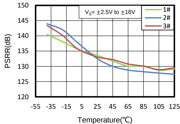
Figure 11. Power-Supply Rejection Ratio vs Temperature
