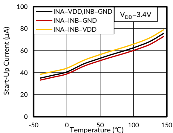
Figure 3. Start-Up Current vs Temperature
