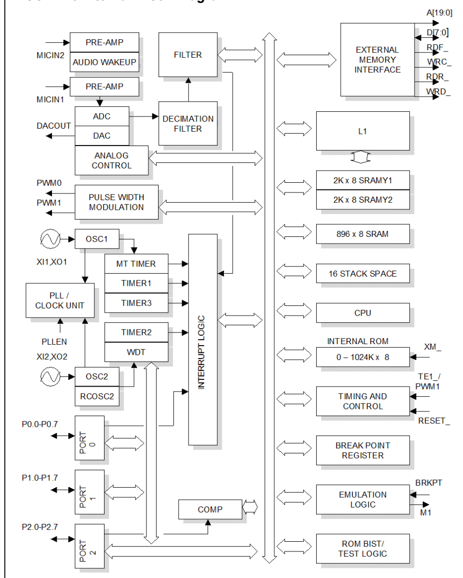
RSC-4128 Internal Block Diagram
