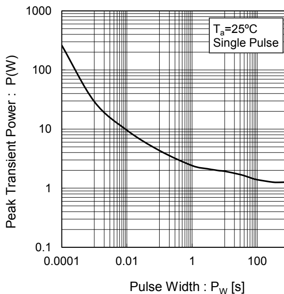
Fig.4 Single Pulse Maxmum Power dissipation
