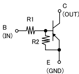
Equivalent circuit
