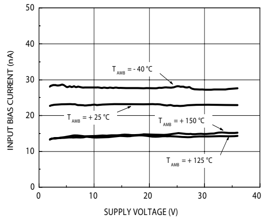
Figure 3: Input current vs. supply voltage
