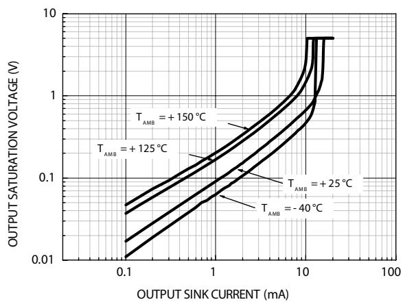
Figure 4: Output saturation voltage vs. output current ( V_{CC} = 5\text{ V} )
